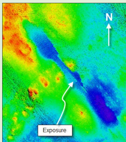
Figure 3.10: Multibeam echo sounder image of a cable exposure along the Gunfleet Sands export cable (source: PLA, 2012)
