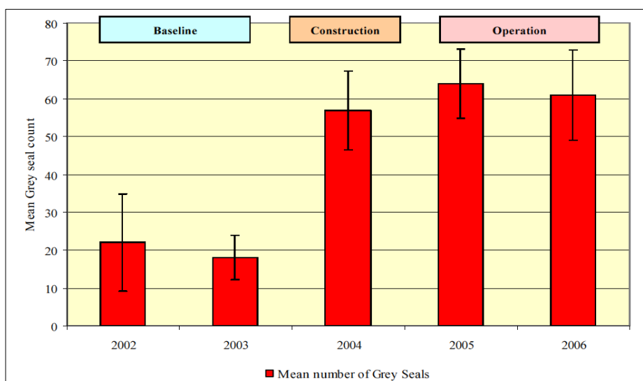
Figure 8.3. Mean abundance of Grey seals recorded during aerial surveys at Scroby Sands Offshore Wind Farm
