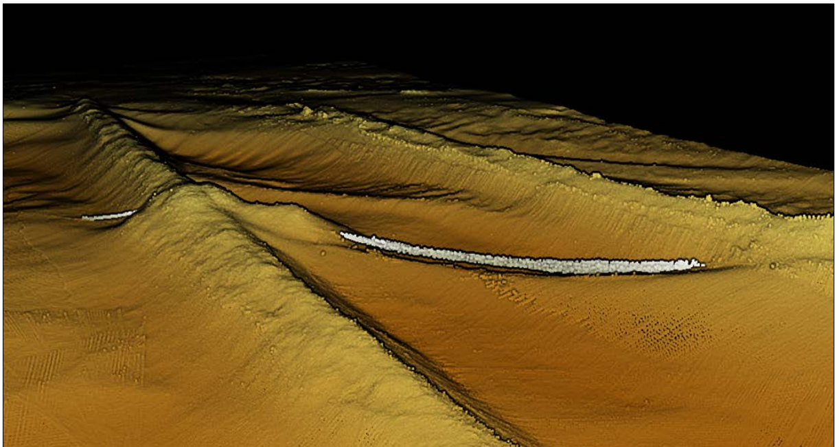
Figure 3.1: Acoustic image of an exposed electrical cable potentially in free-span at the location of a cable crossing
