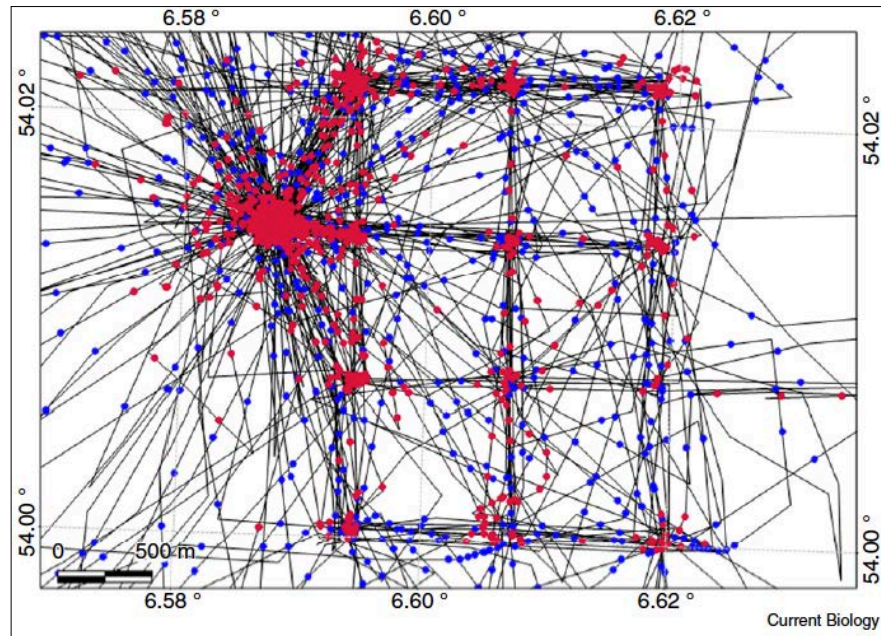
Figure 6.7: The tracks of a harbor seal around Alpha Ventus Offshore Wind Farm
