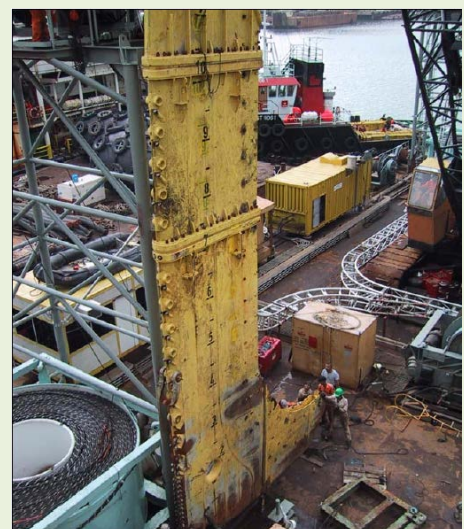
Vertical injector tool (source: CMACS, 2006)
