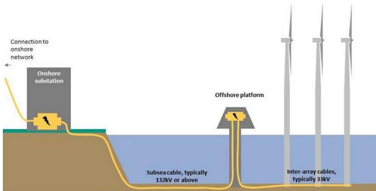
Figure 1. Offshore Wind Electric Cable Schematic from Turbines to Onshore Grid Connection
