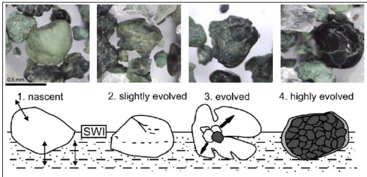
Figure 2. Glaucanite Morphology
