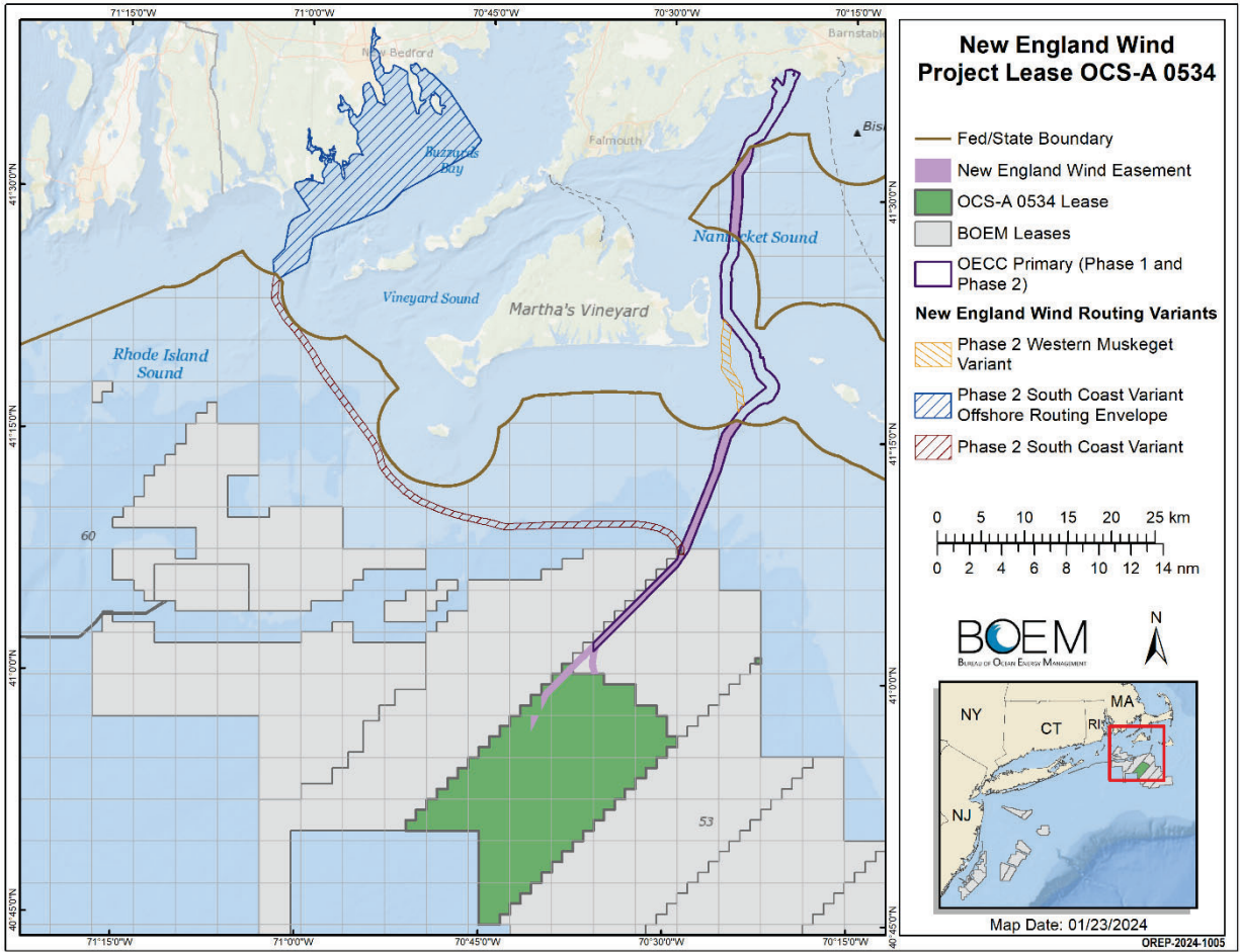
Figure 2: Project Overview – Lease Area and Submarine Export Cable Routes
