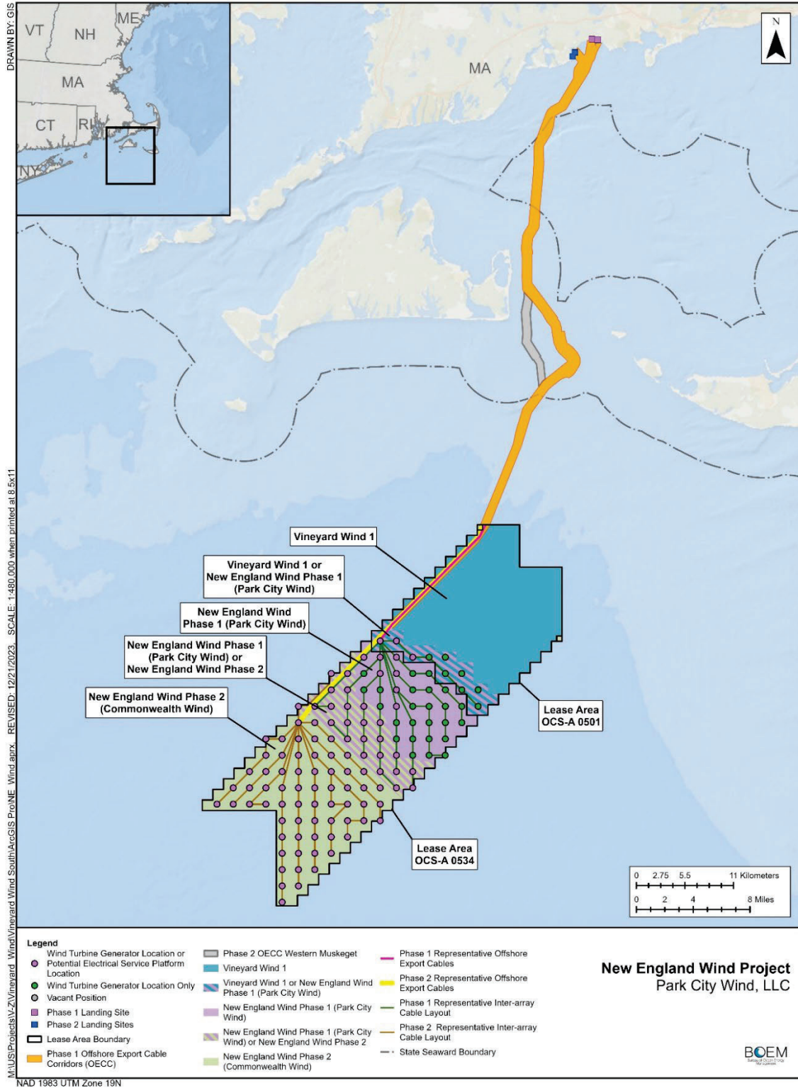
Figure 1-1: Project Area and Facilities
