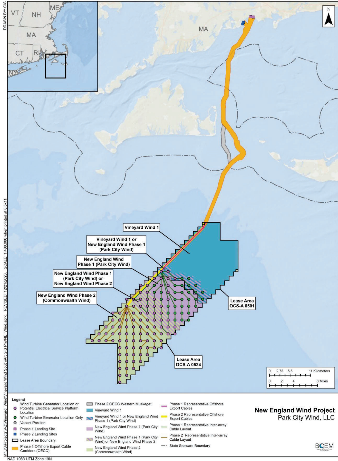
Figure 1: Lease Overview – Lease Segregation and Phase Details
