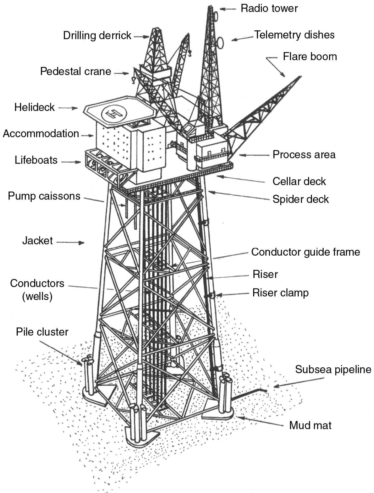
FIGURE 1-2 Typical Offshore Jacket Structure Designed for Use in 350 ft (107 m) of Water (Source: PetroWiki 2015).
