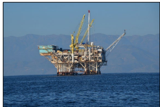
FIGURE 3.13-3 Santa Barbara Channel.
