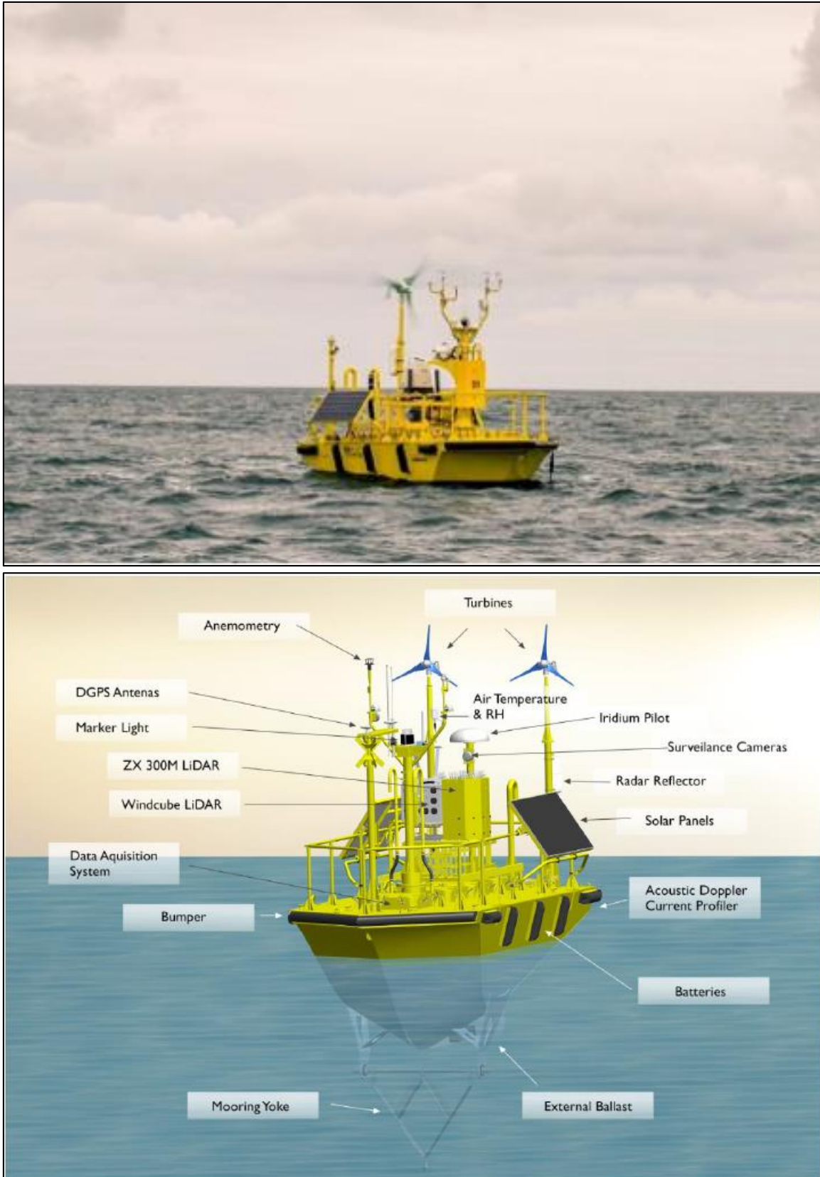
Figure 2-1 Typical AXYS WindSentinel™ Environmental Monitoring Buoy
