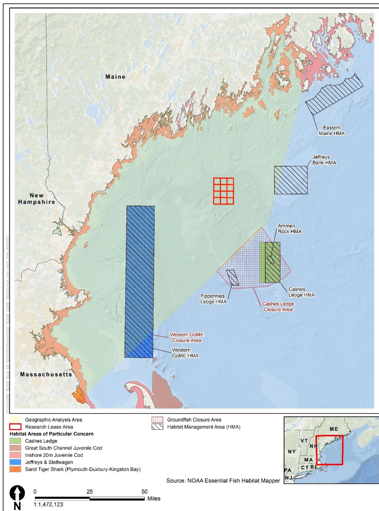
Figure 3-2. Habitat areas of particular concern in the vicinity of the Research Lease Area within the Gulf of Maine
