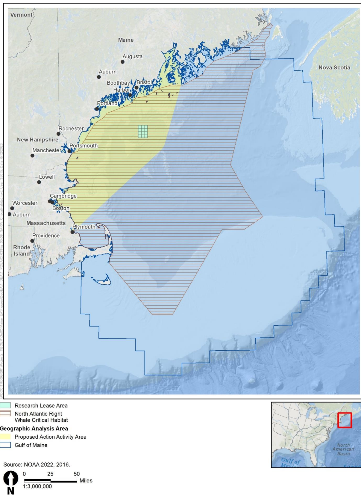
Figure 3-3. North Atlantic right whale northeastern critical habitat within the Gulf of Maine
