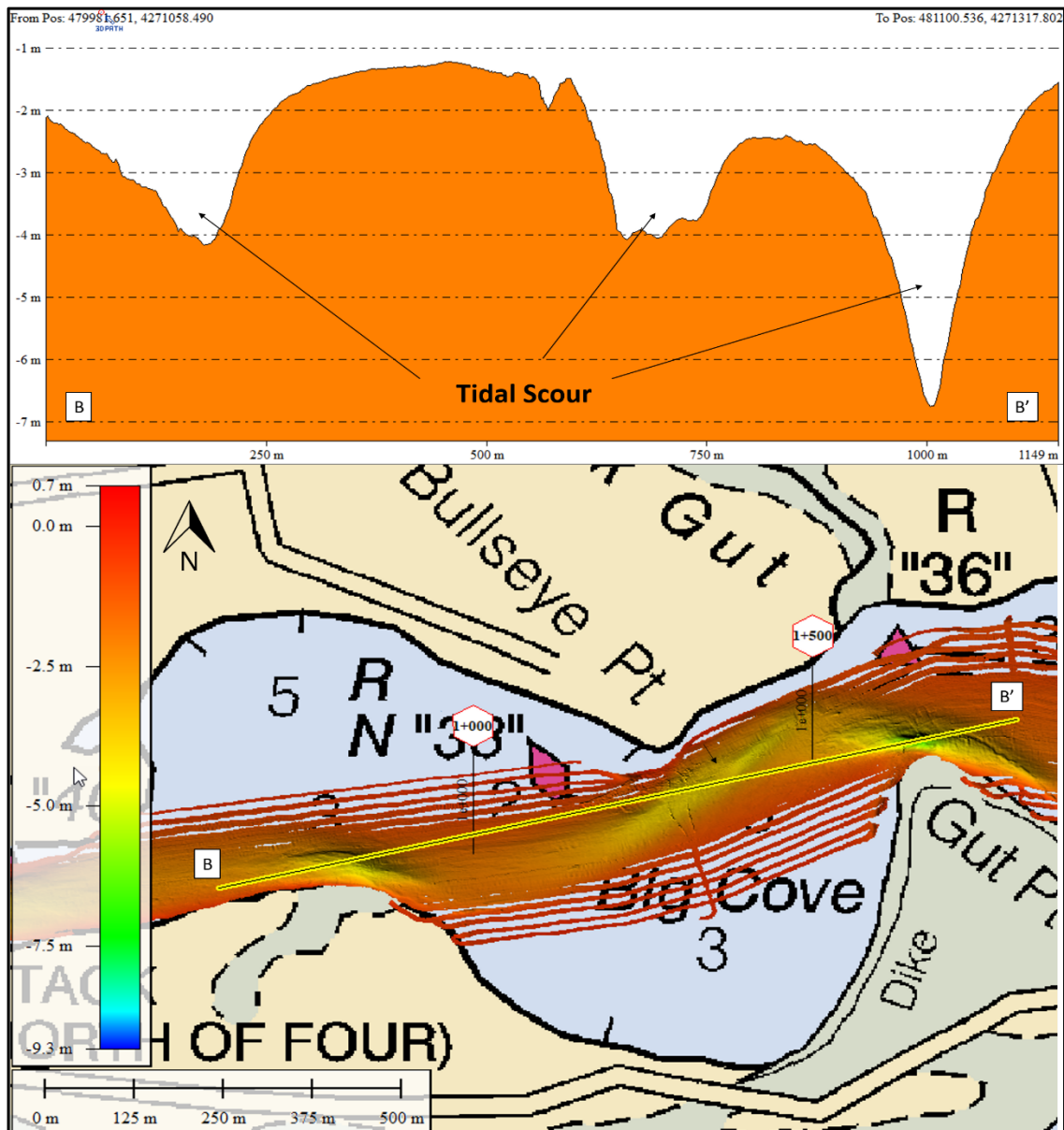
Figure 10.2 Bathymetry data illustrating tidal scouring along the Indian River
