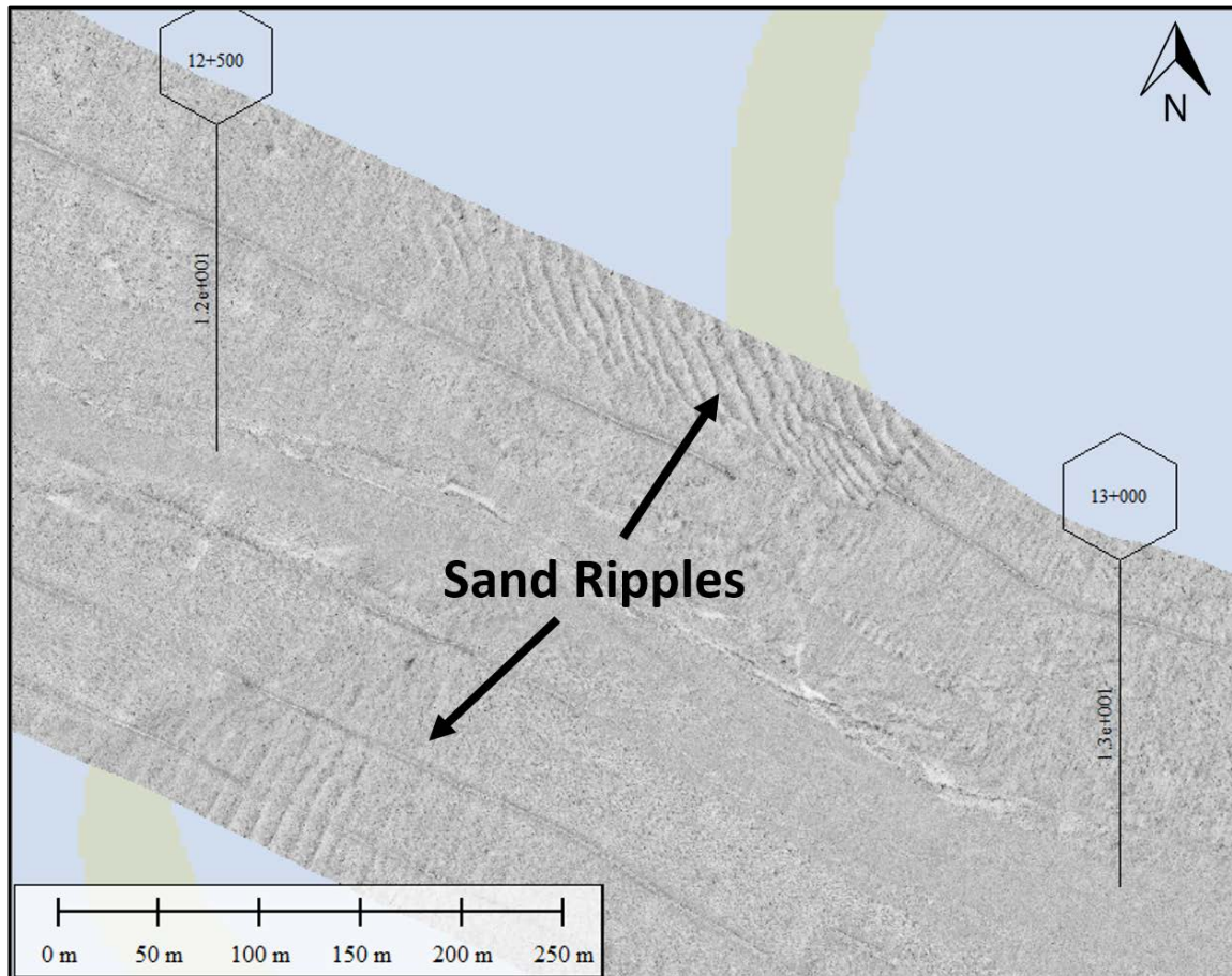
Figure 10.8 Section of the sonar mosaic showing sand ripple areas between KP 12+500 and 13+000
