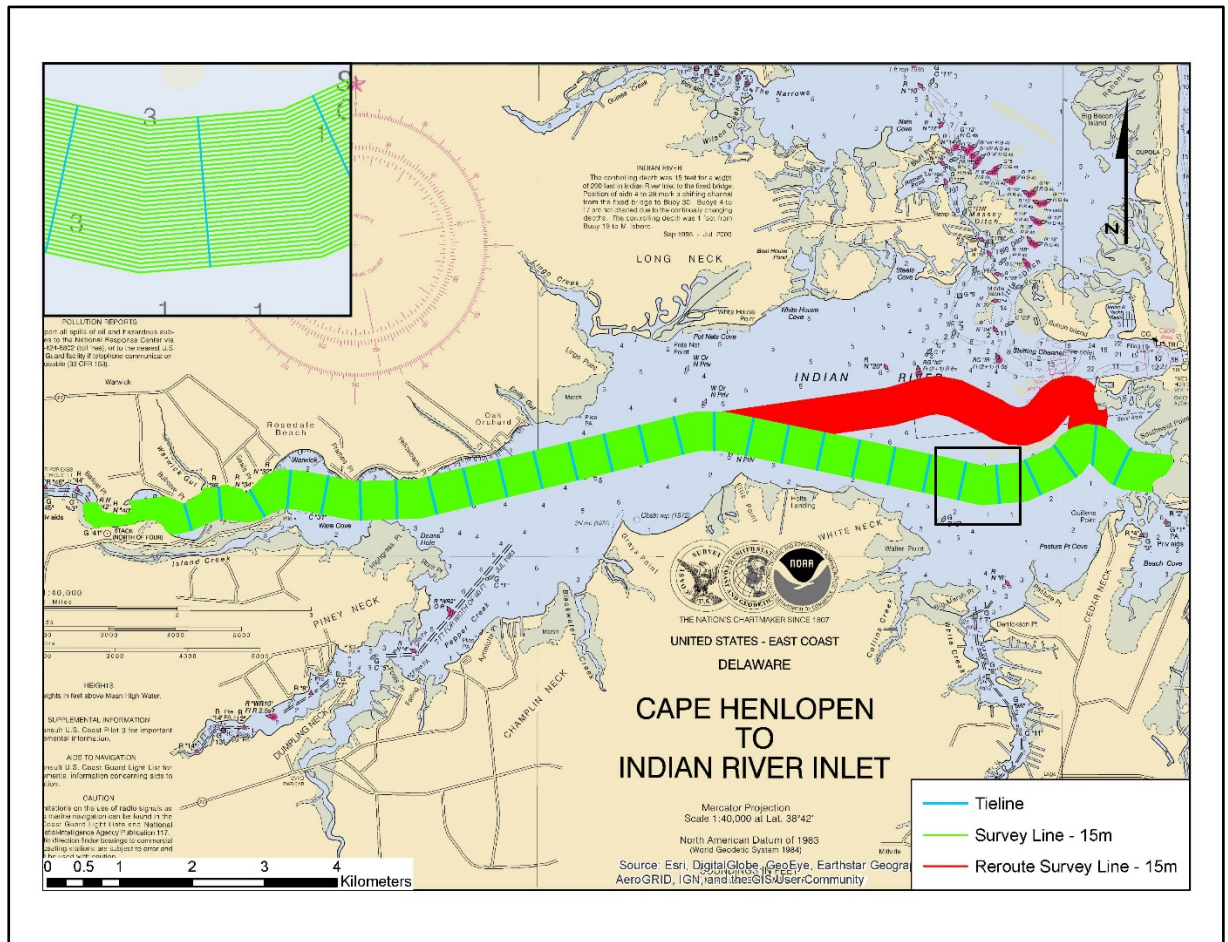
Figure 6.2 Inshore export cable survey line plan with reroute
