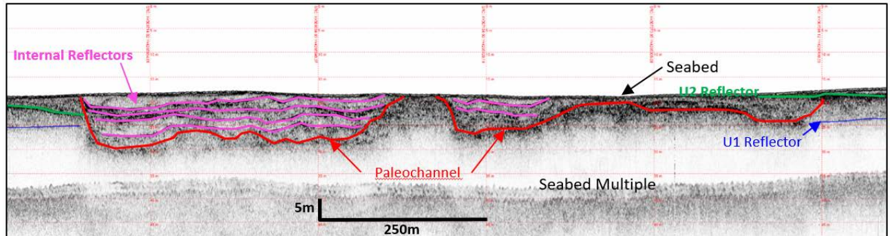
Figure 9.11 Paleochannel between KP 12+800 – 13+900
