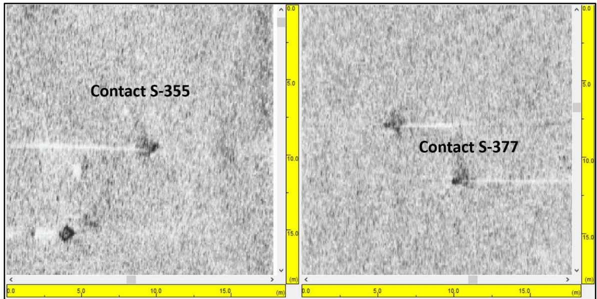
Figure 10.3 Side scan Imagery of two sonar contacts with greater than 1 m relief between KP 0+000 and KP 9+000
