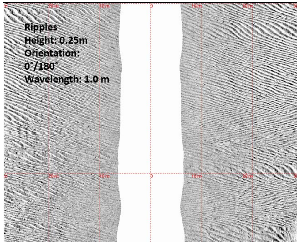
Figure 9.6 Sand Ripples between KP 0+000 – 0+500
