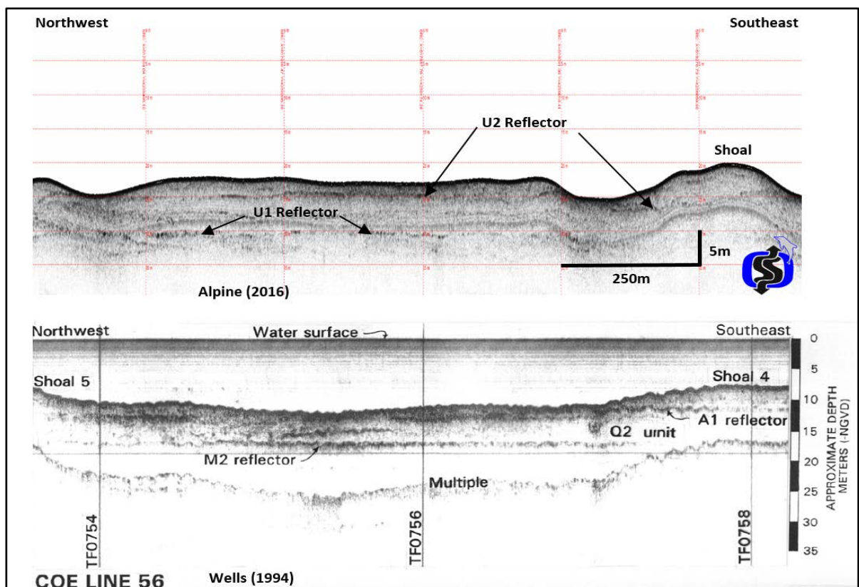
Figure 9.2 Comparison of Sub-bottom Reflectors
