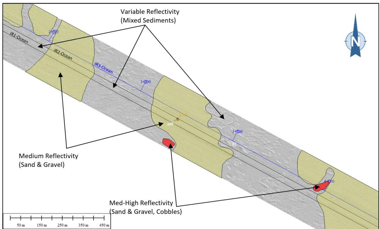
Figure 9.7 Side Scan Sonar Mosaic with Seabed Classification, KP 2+500 – 4+300
