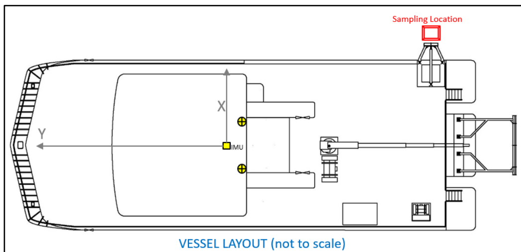
Figure 6.5 Sampling equipment configuration
