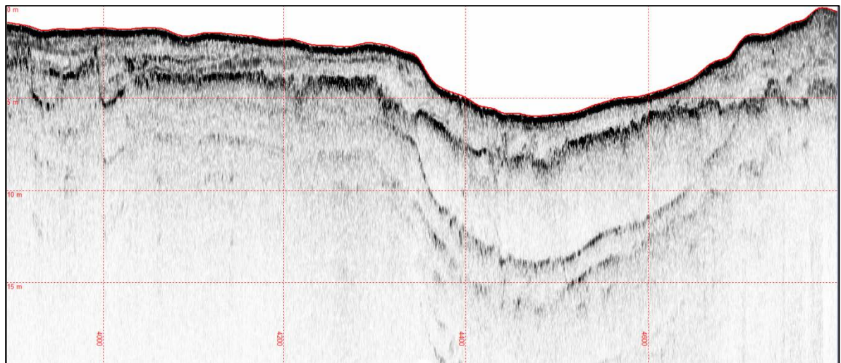
Figure 6.7 Edgetech 3100P data example showing seafloor penetration
