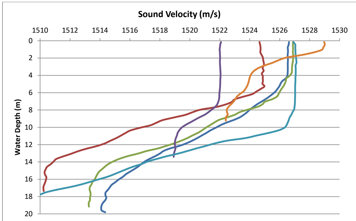
Figure 6.4 Example of SVP profiles collected during the offshore HRG survey
