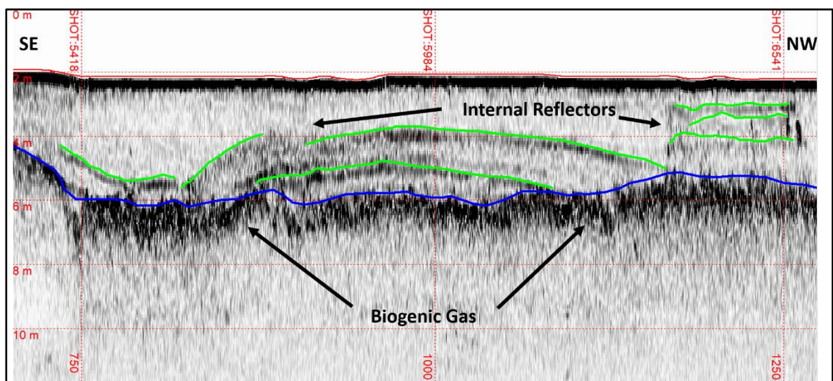
Figure 10.1 Sub-bottom profile showing reflector types on inshore cable route
