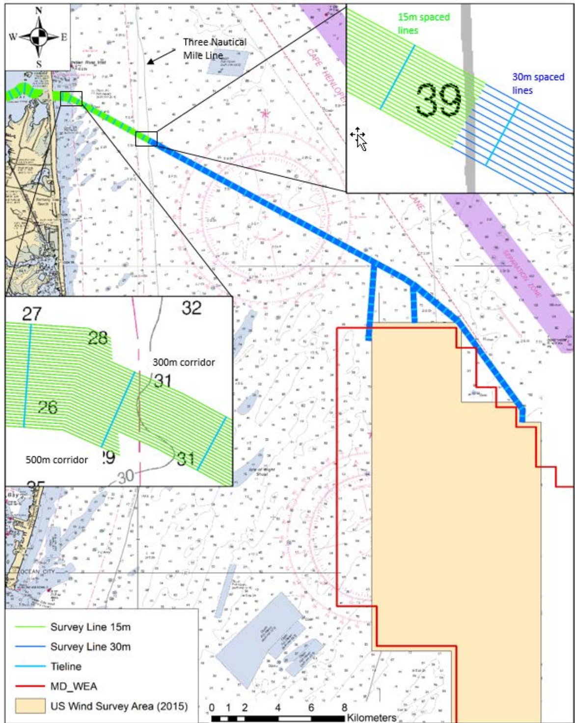
Figure 6.1 Offshore export cable survey line plan
