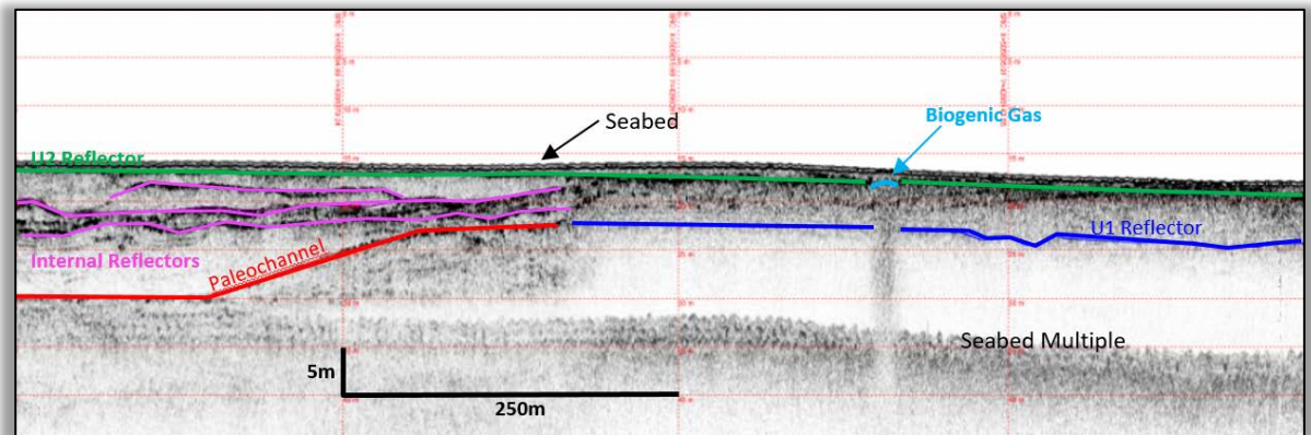
Figure 9.3 Sub-bottom Profile with Mapped Reflectors
