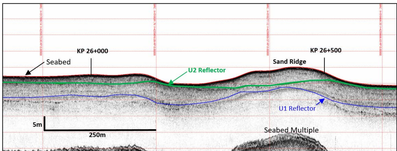
Figure 9.15 Sub-bottom Profile showing Sand Ridge
