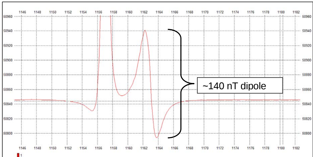
Figure 6.8 Geometrics G-882 Magnetometer Data Example
