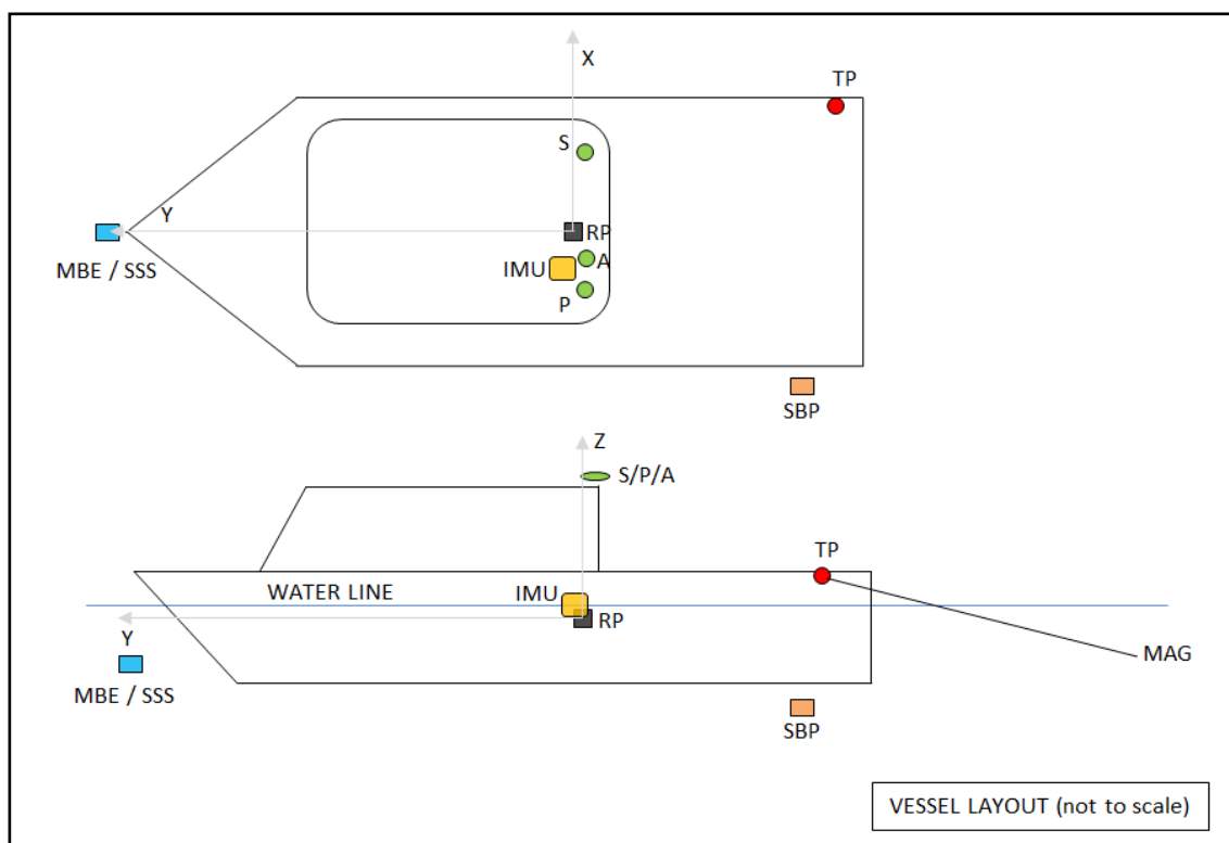
Figure 6.7 MV William M Offset diagram
