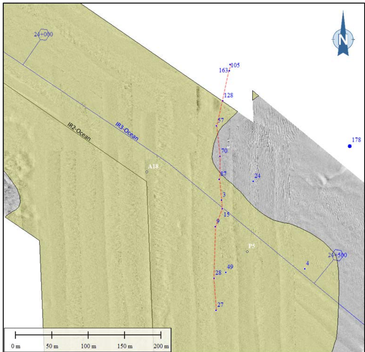
Figure 9.13 Linear Arrangement of Magnetic Anomalies near KP 24+300
