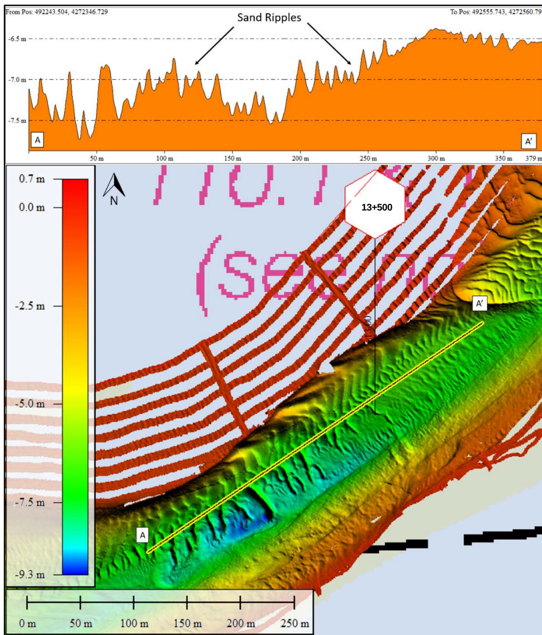
Figure 10.6 Bathymetry data showing sand ripples near Indian River bay Inlet
