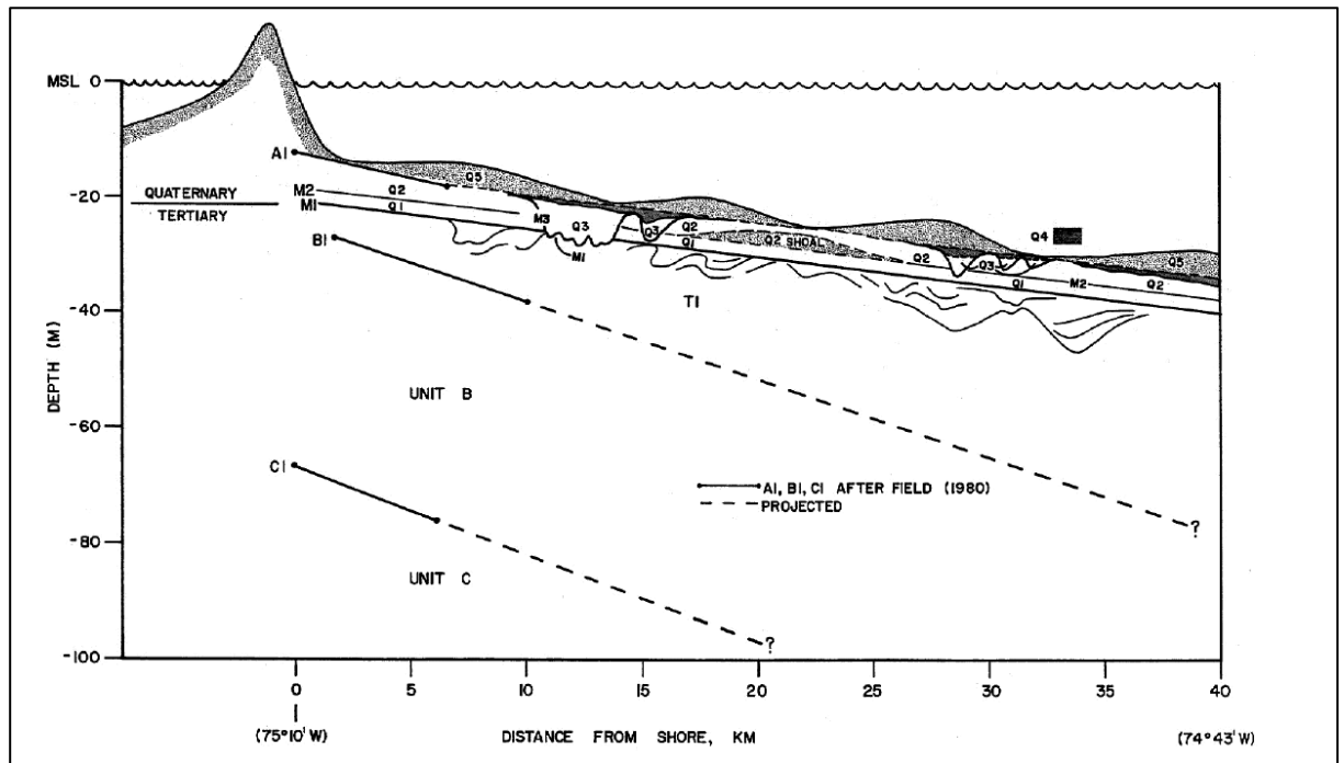
Figure 7.3 Maryland's Inner Continental Shelf Stratigraphy (from Toscano et al. 1989)
