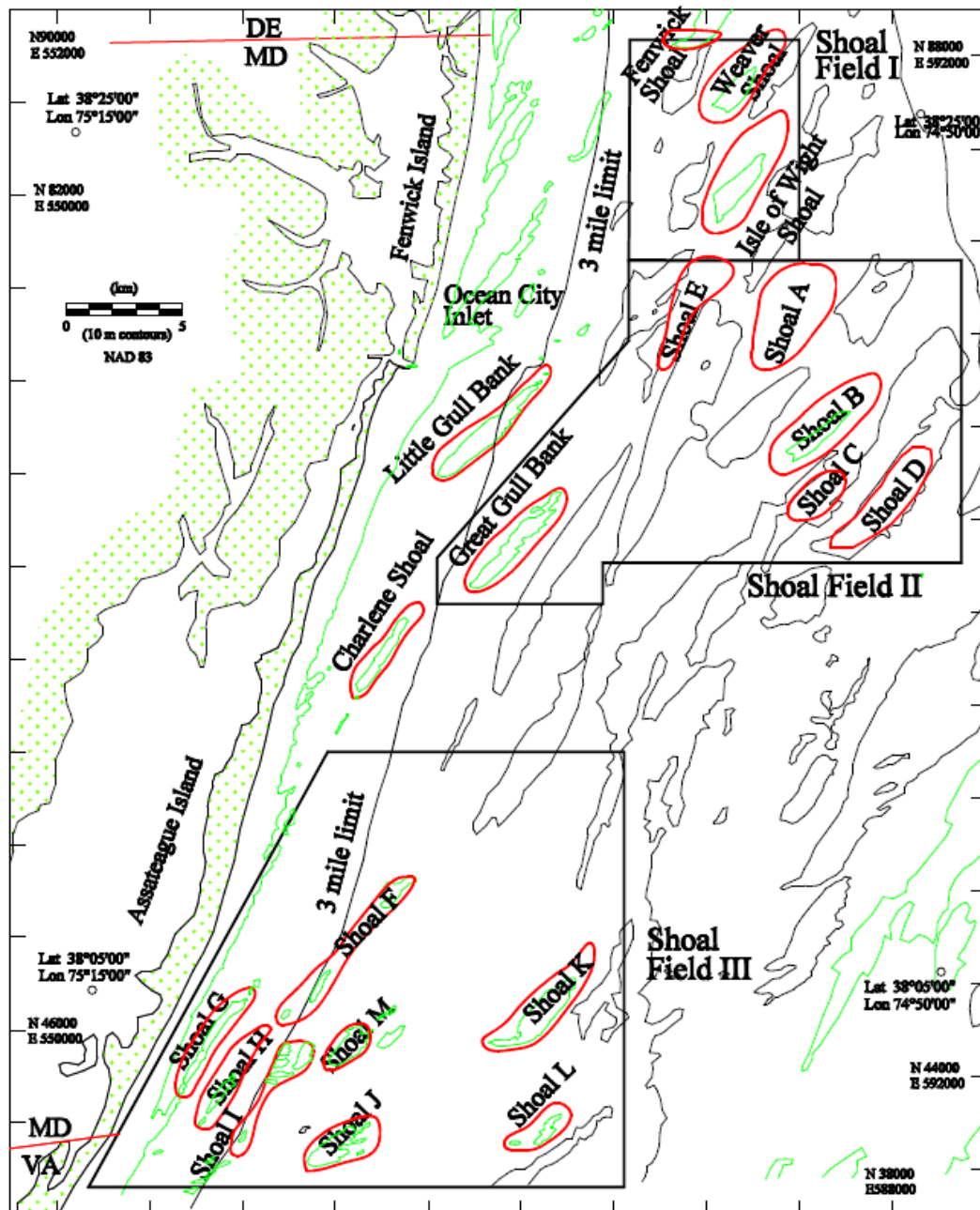
Figure 7.2 Index of Shoal fields Offshore Maryland
