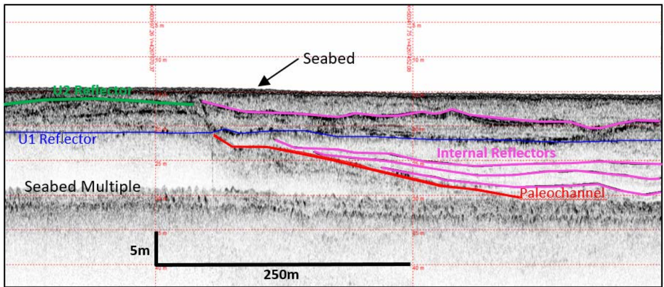
Figure 9.10 Northwest Flank of Paleochannel near KP 9+000
