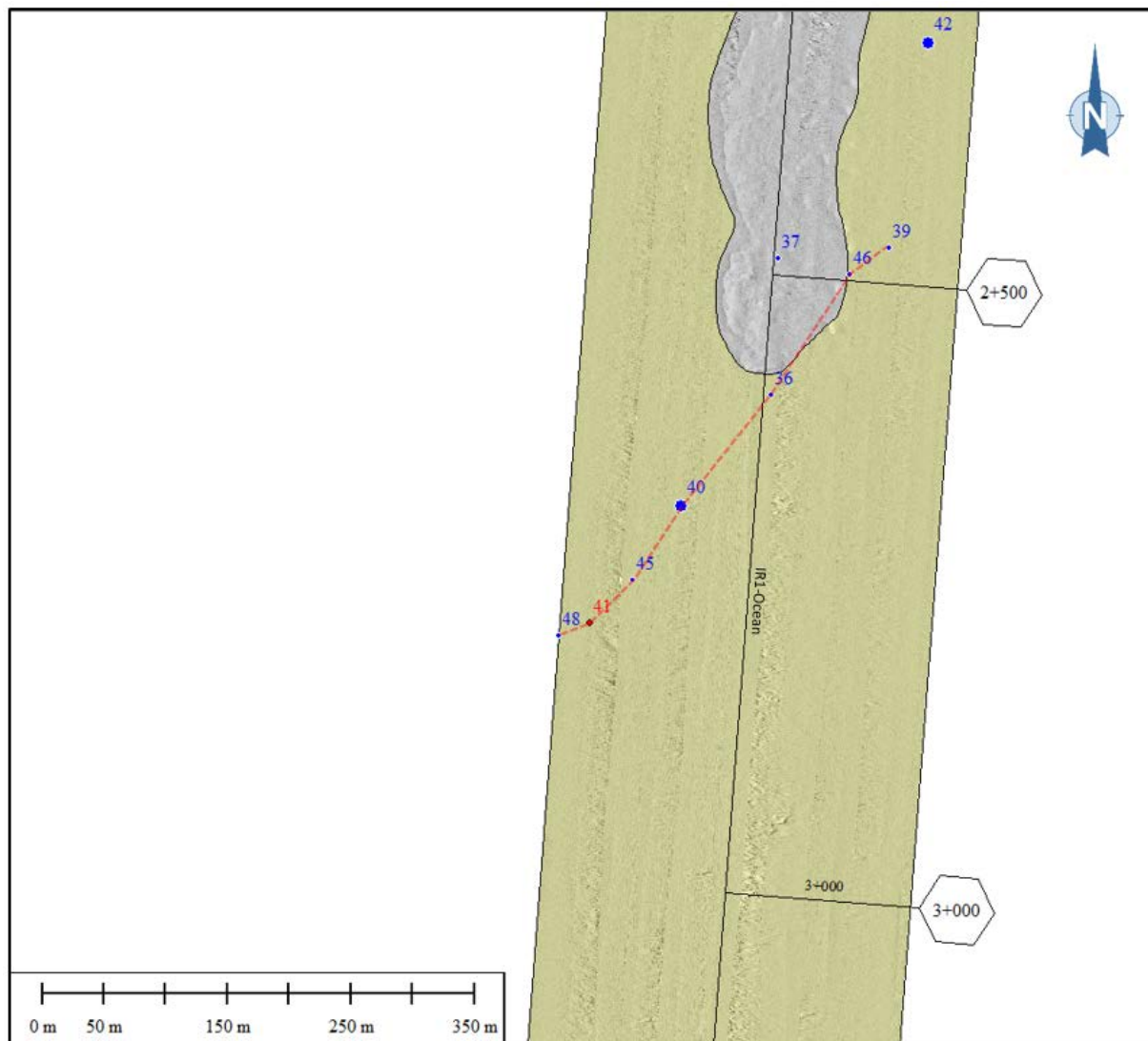
Figure 9.16 Linear Arrangement of Magnetic Anomalies along IR1-Ocean Extension
