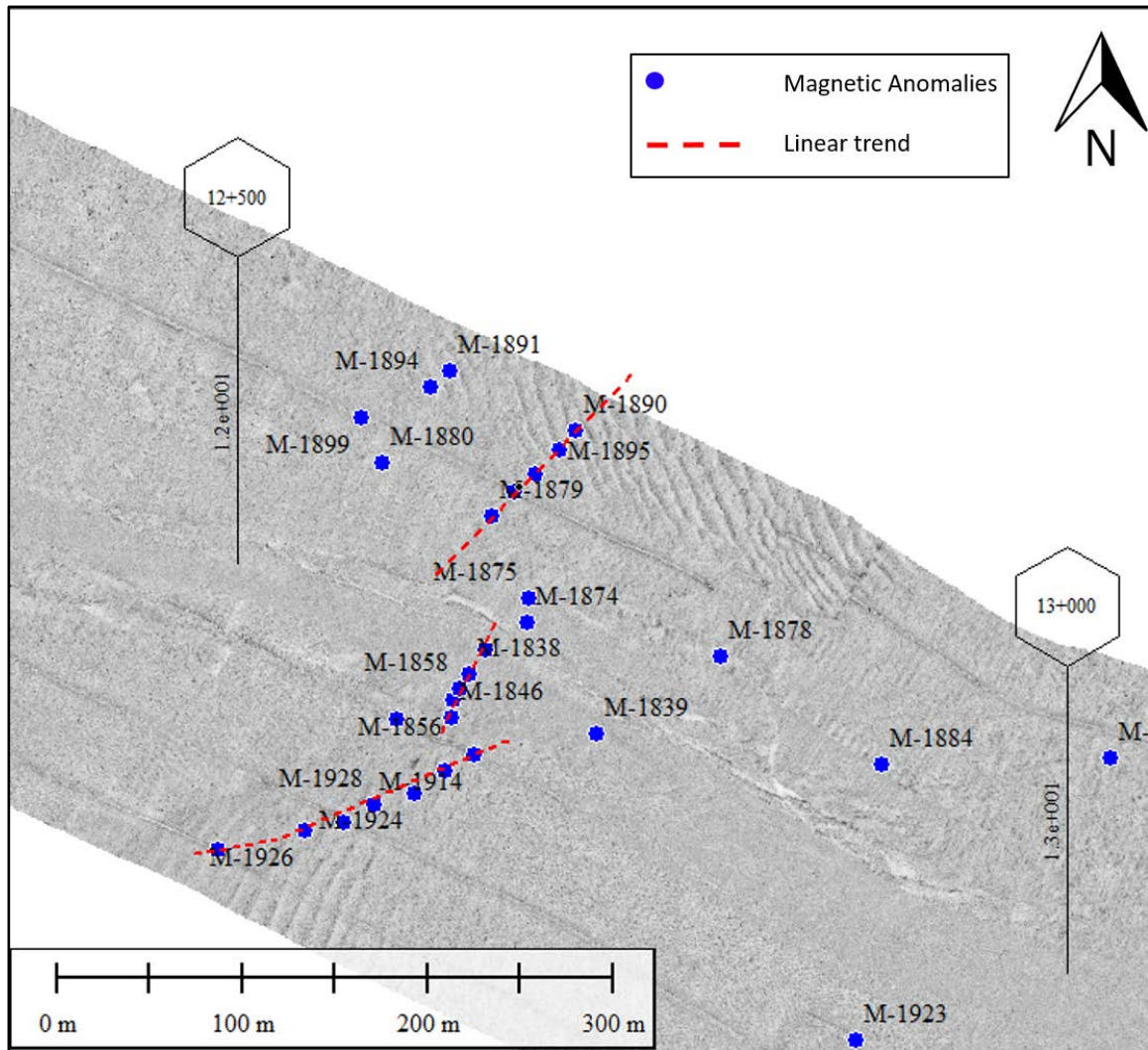
Figure 10.9 Image showing linear trends in magnetic anomalies between KP 12+500 and KP 13+000
