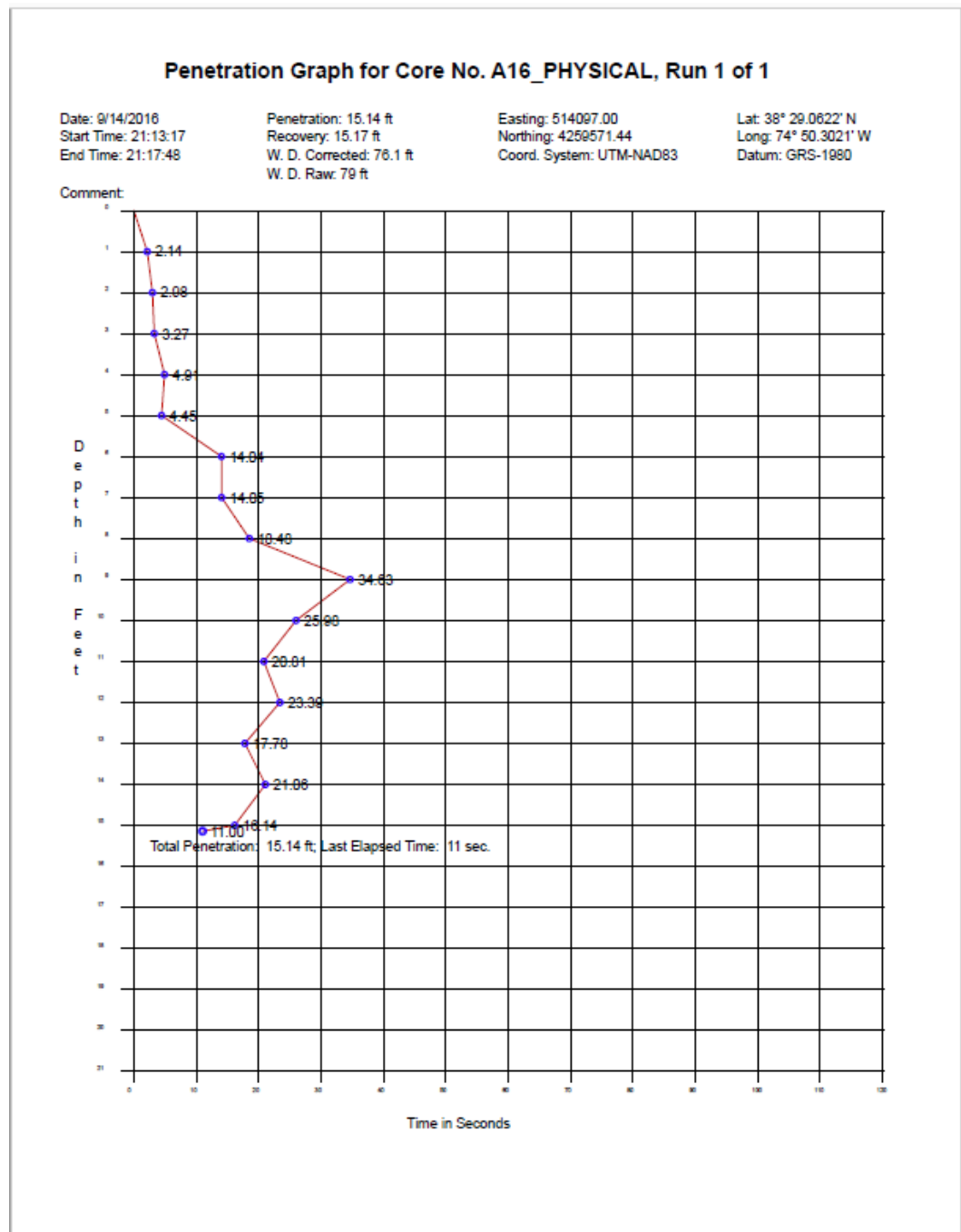
Figure 6.6 Example of a Penetration Graph
