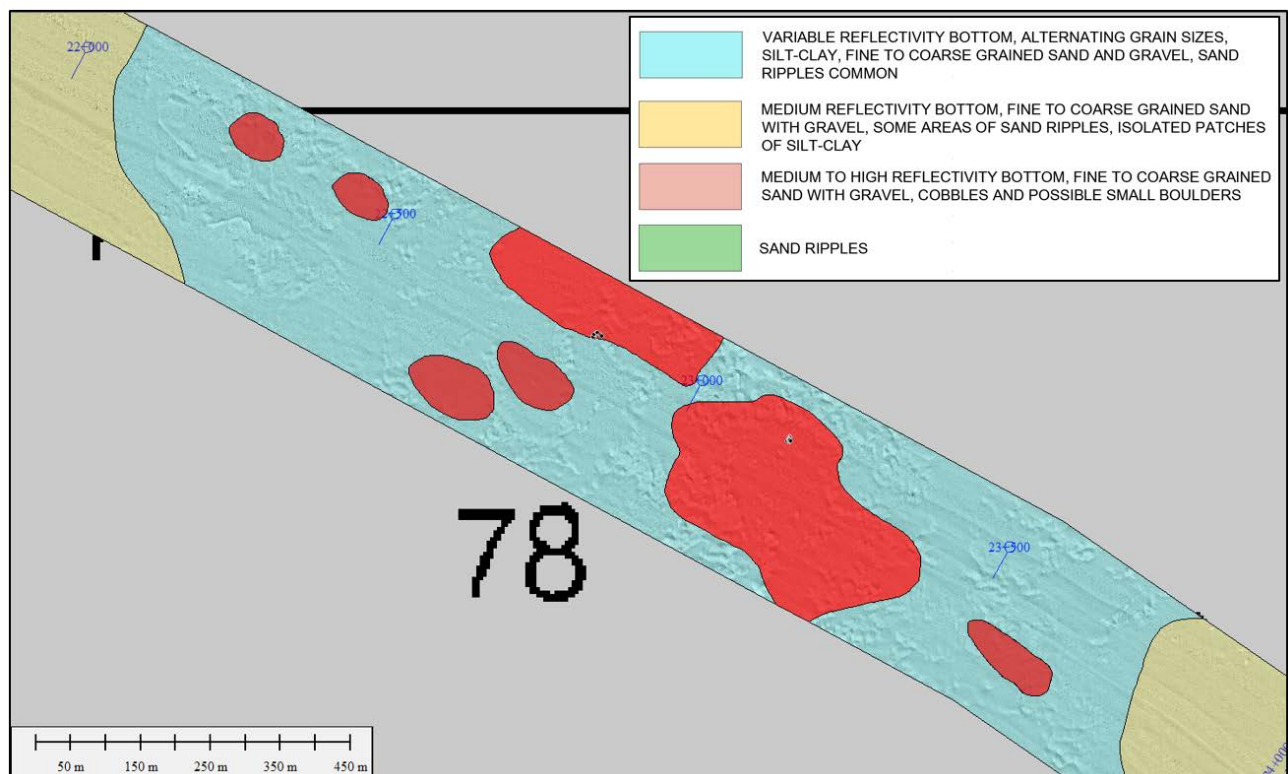
Figure 9.1 Side Scan Sonar Mosaic with Seabed Classification
