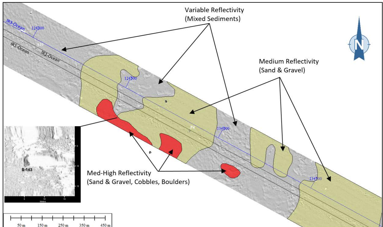
Figure 9.9 Side Scan Sonar Mosaic with Seabed Classification, KP 12+000 – 13+800
