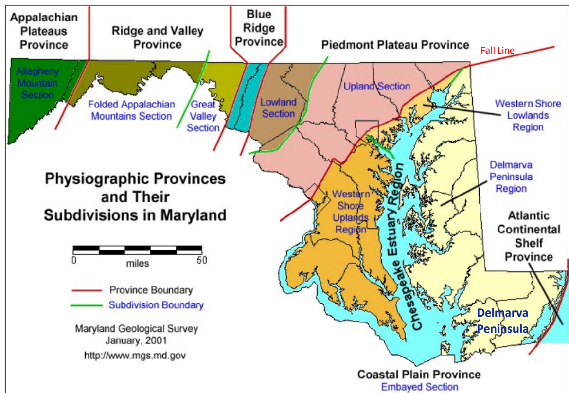
Figure 7.1 Maryland Physiographic Provinces (modified from the USGS)
