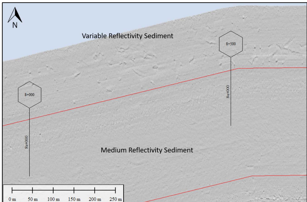
Figure 10.4 Section of the sonar mosaic showing sediment characterization between KP 8+000 and KP 8+500
