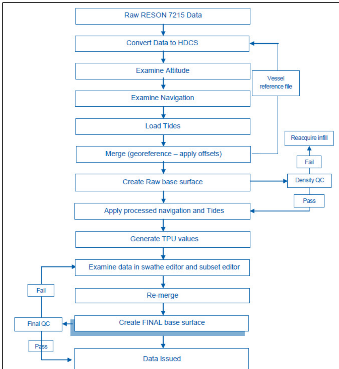
Figure 8.1 MBES processing flow diagram for bathymetry data
