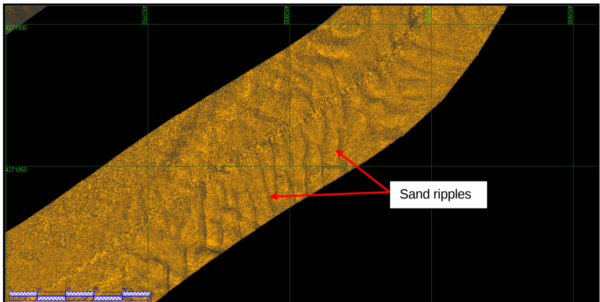
Figure 6.6 Edgetech 6205 SSS Data Example
