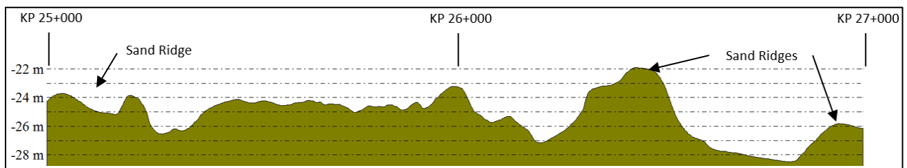
Figure 9.14 Sand Ridges between KP 25+000 – 27+000
