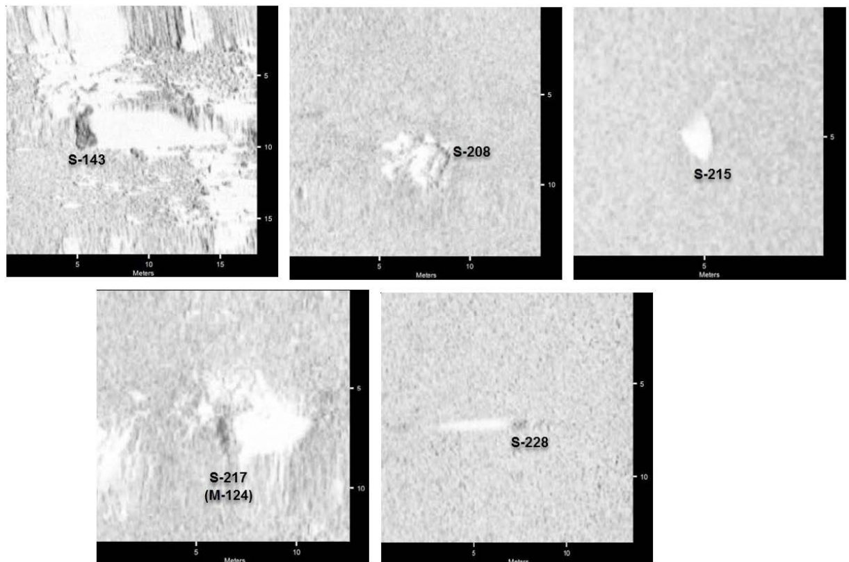
Figure 9.8 Significant Side Scan Sonar Contacts Identified between KP 7+500 – 18+000
