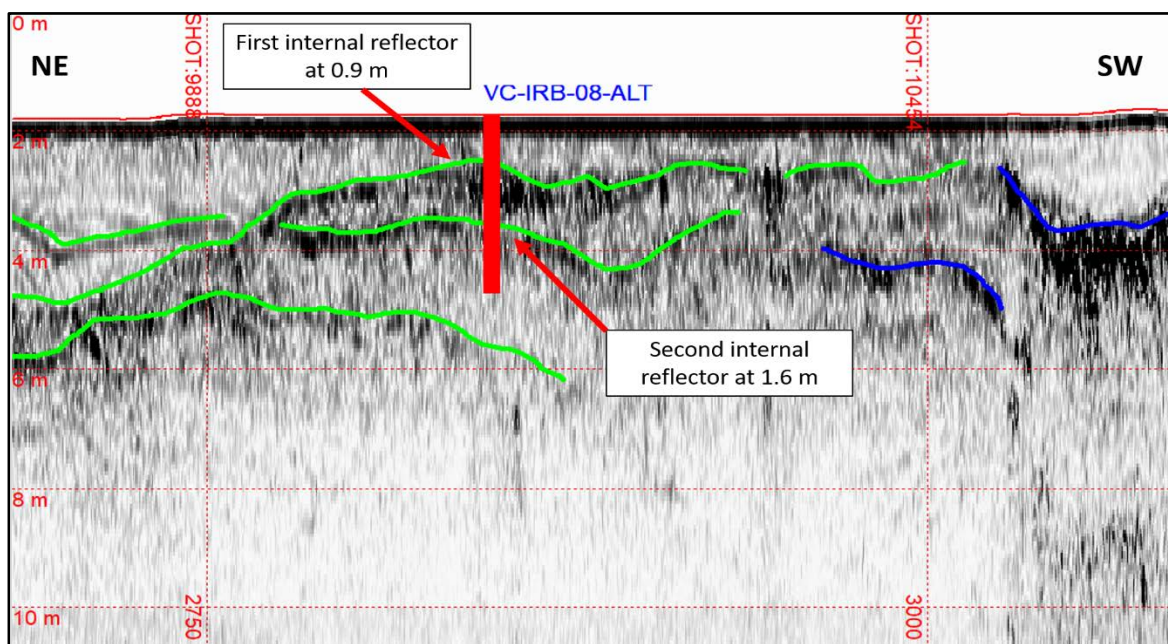
Figure 10.5 Sub-bottom profile showing internal reflectors near core location VC-IRB-08-ALT
