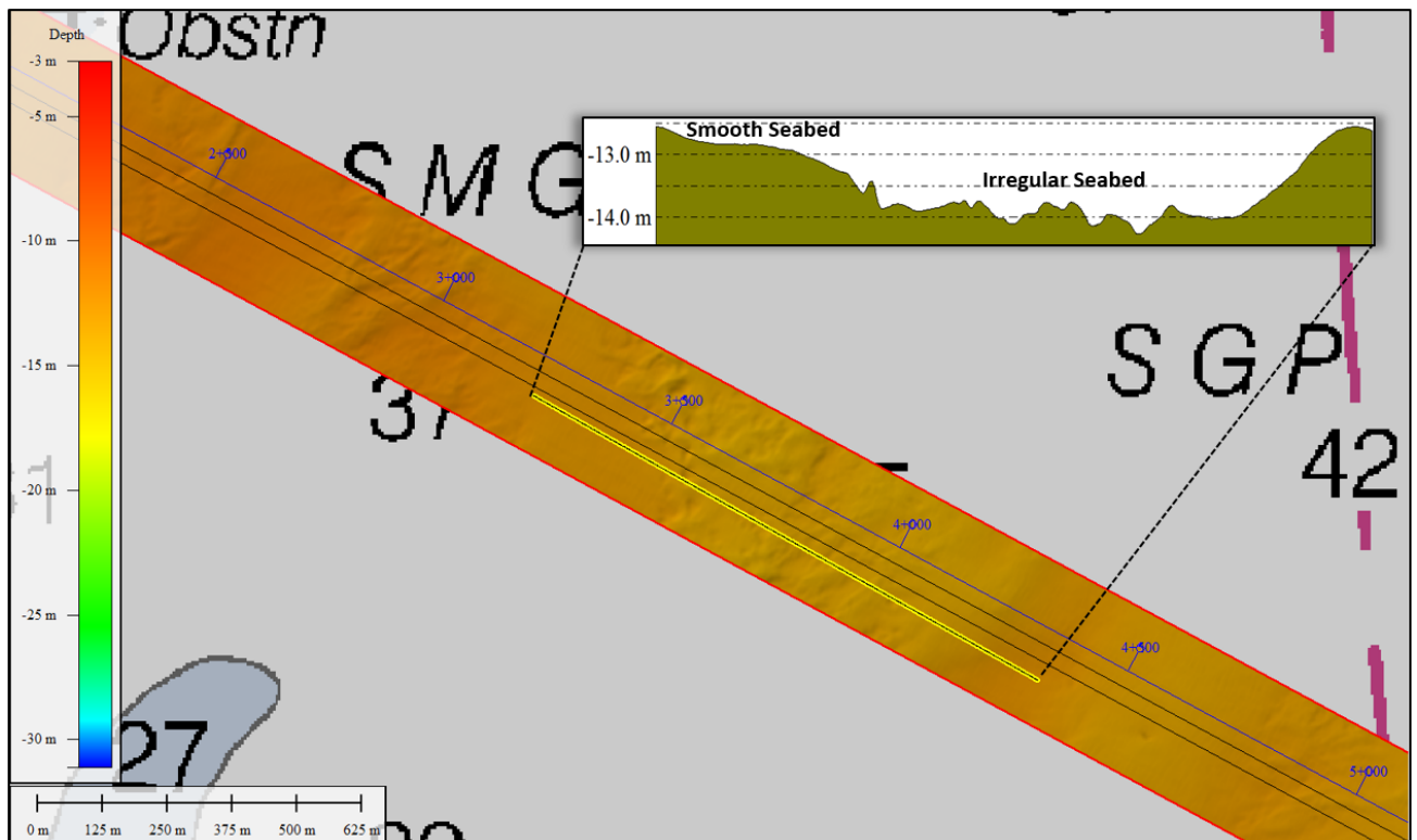
Figure 9.4 Bathymetry between KP 3+000 – 4+500 Showing Transition From Smooth to Irregular Bottom
