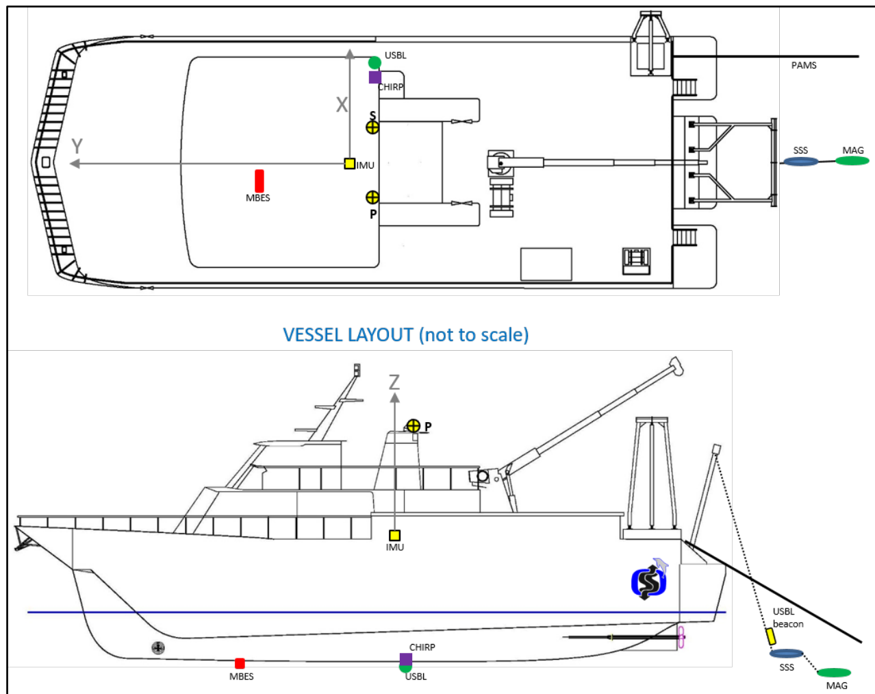
Figure 6.3 RV Shearwater HRG Offset Diagram
