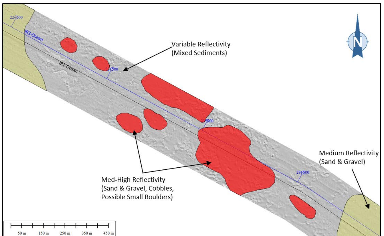
Figure 9.12 Side Scan Sonar Mosaic with Seabed Classification, KP 22+000 – 23+900
