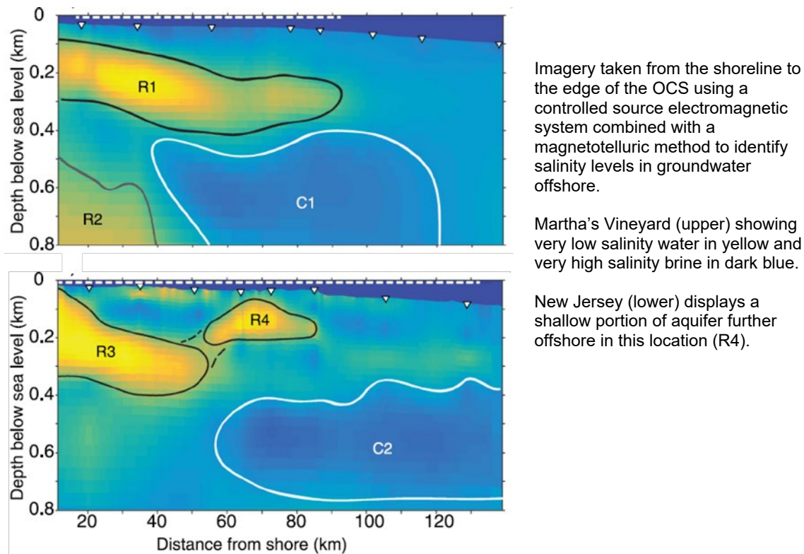
Figure 6. Imagery of Cross-sections of Martha's Vineyard and New Jersey Offshore Aquifers (Gustafson, et al., 2019)
