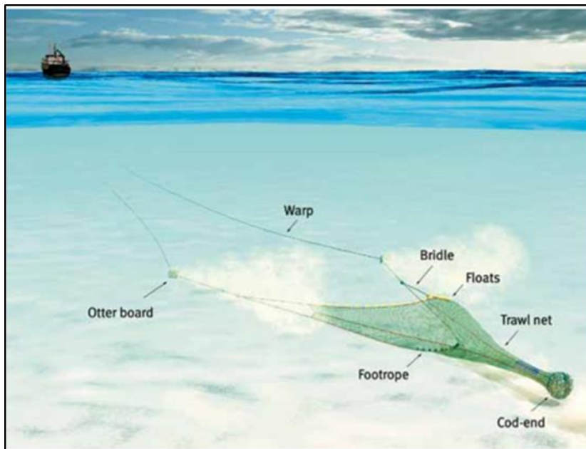
Figure 2.3: Example of a bottom trawl configuration and otter boards.
