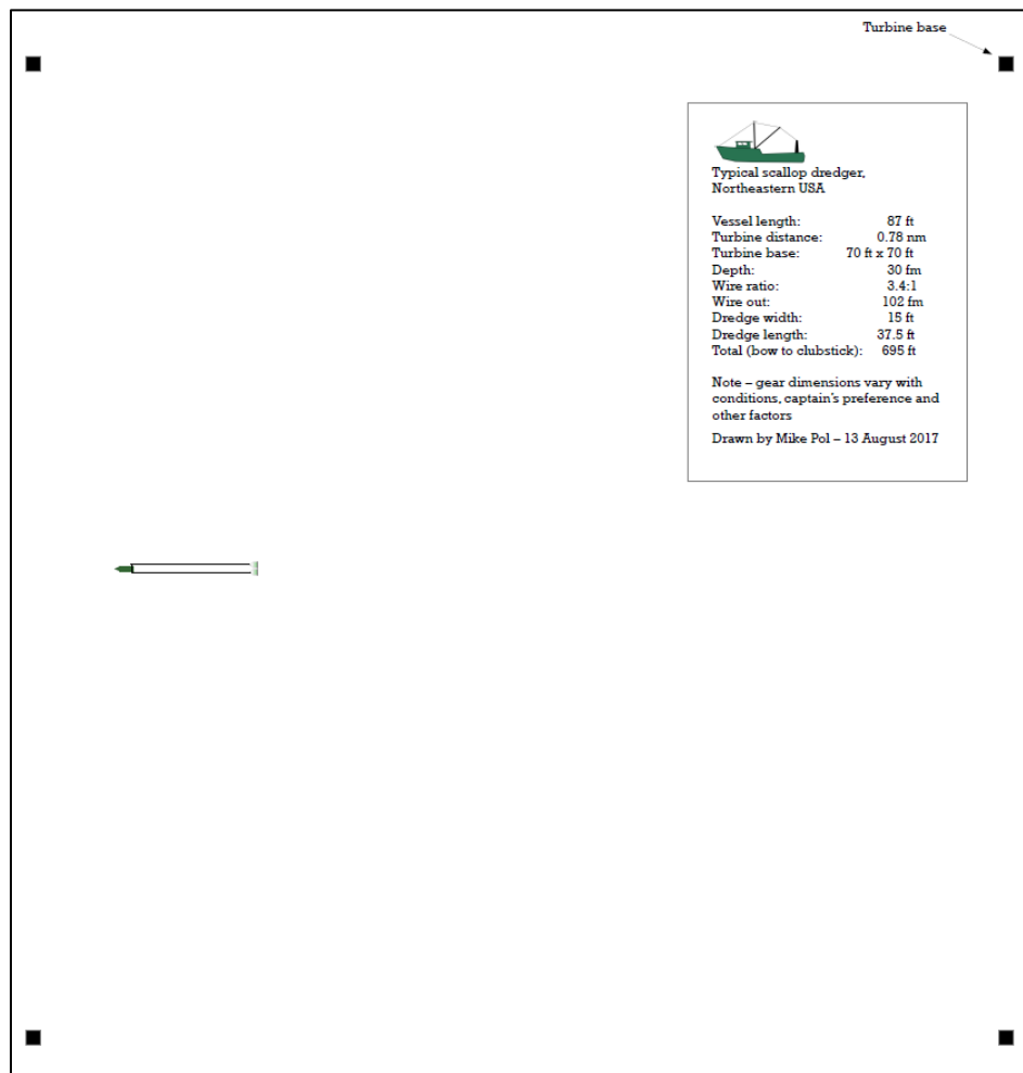
Figure 2.28: Scale drawing represents 87' scallop dredge vessel working a depth of ~180' (~55m) within turbines at 0.78 nm spacing; drawing represents turbine base of 70' x 70'. (Source: NYSEDA Offshore Wind Master Plan 2017)
