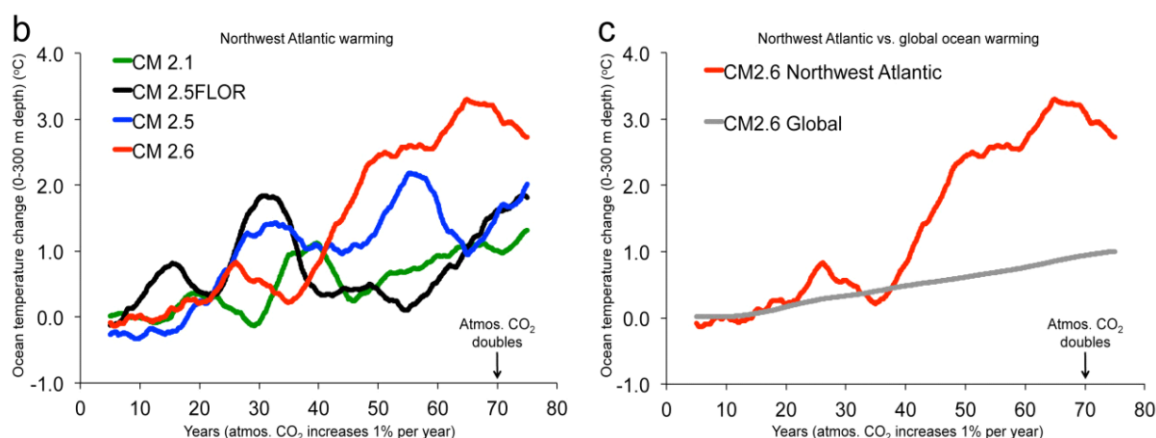
Figure 3-18. Ocean Warming Modelled in the Northwest Atlantic (left panel) and Compared to Global Averages (right)
